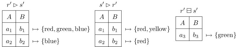
Fig. 2. Example of the derived color algebra operators \triangleright (Example 2) and tuple difference ( \ominus ) (Example 4) on the two color relations r' and s' given in Fig. 1.
