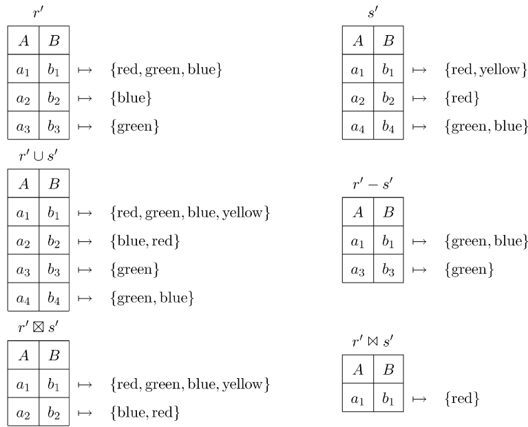
Fig. 1. Example of the color algebra operators union ( \cup ), full difference ( - ), tuple join ( \boxtimes ) and full join ( \bowtie ) on two color relations r' and s' .
